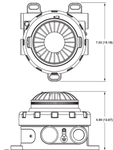
Figure 2—U5015 Dimensions in Inches (cm)
