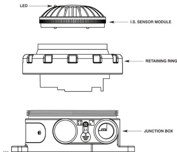
Figure 1—U5015 Components
